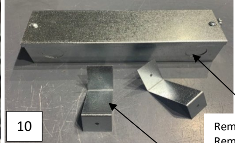
Z Bracket (Typ. 2)
