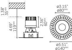
Round Trimless
