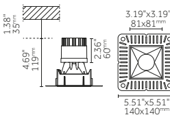
Square Trimless
