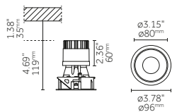
Round Trimless
