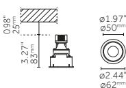
Round Trimless
