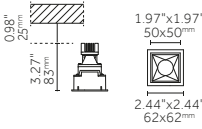
Square Trimless
