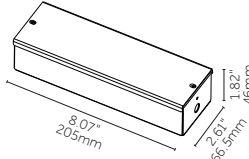
Remote Driver
