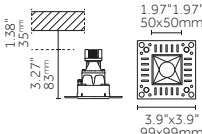
Square Trimless
