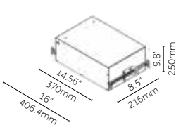
IC/AT/CP Housing Large
