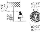
Round Trimless
