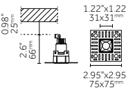
Square Trimless
