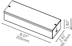
Remote Driver
