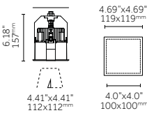
Square Trimless
