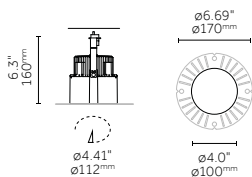
Round Trimless
