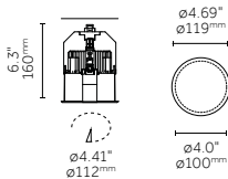
Round Trimless
