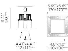
Square Trimless
